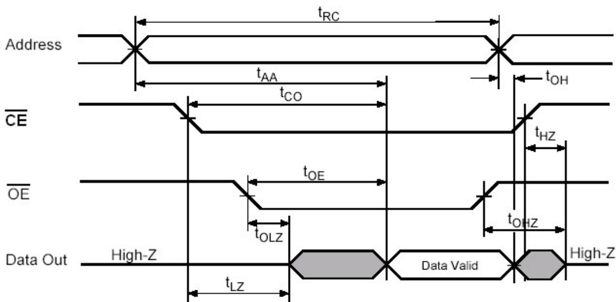
READ CYCLE(2) (/OE Controlled)
