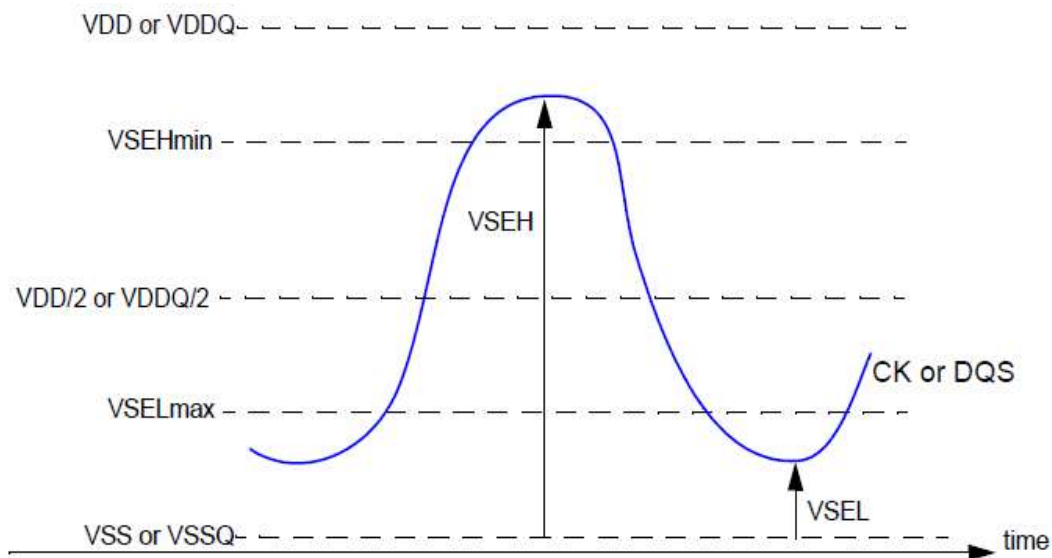
Single-ended requirement for differential signals.
