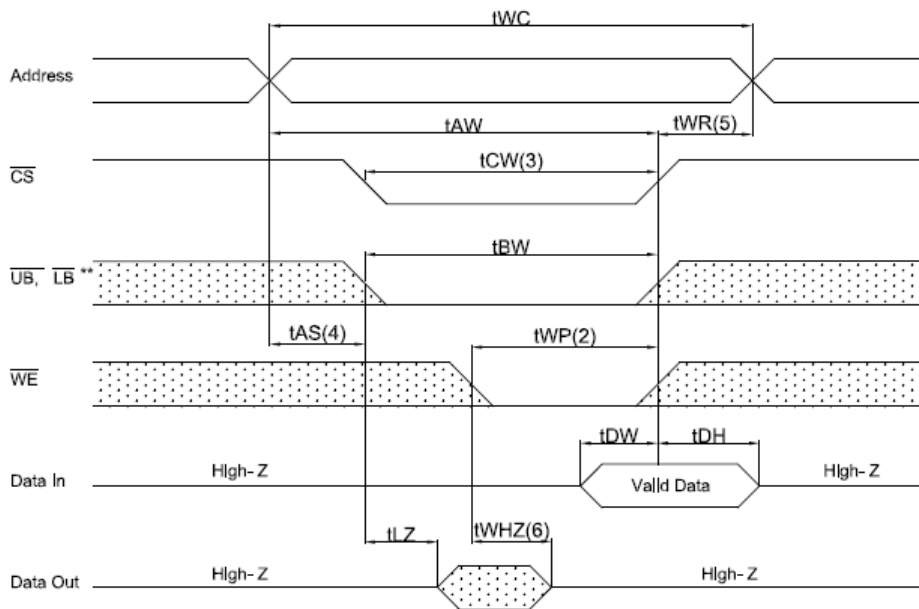
Timing Waveform of Write Cycle (3) ( \overline{CS} = Controlled)
