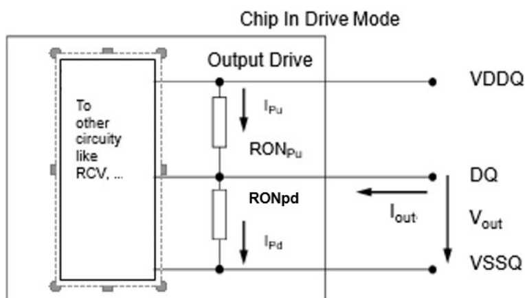
Figure 15. Output driver
