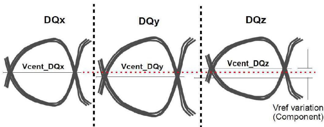
Figure 25. Vcent_DQ Variation to Vcent_DQ(midpoint)
